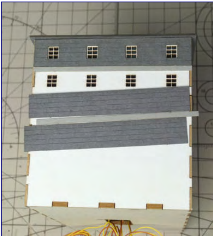
According to the instructions, the gable walls are glued first, then the sides. In order to have a contact edge for the alignment, we work our way through the facade parts from top to bottom.
