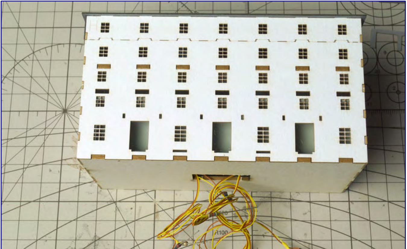
After the interior lights are mounted, the cables are fed through the base plate to the outside. Now we continue with the design of the façade.
