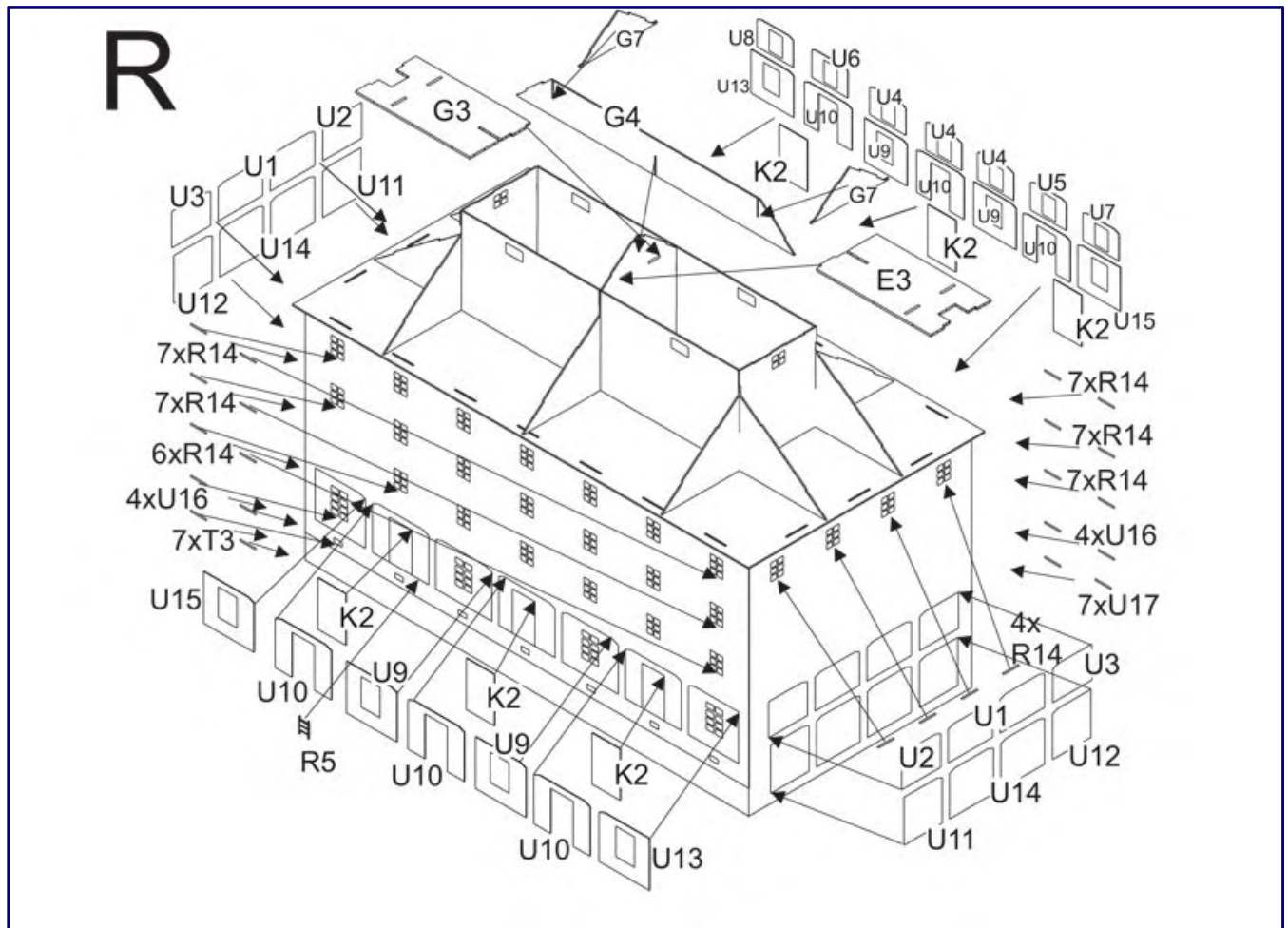
Don't be scared. Construction step R appears overloaded with parts. A closer look reveals that this is due to the large number of window sills that distort the diagram somewhat. Photo: Modellbau Laffont / Märklin
