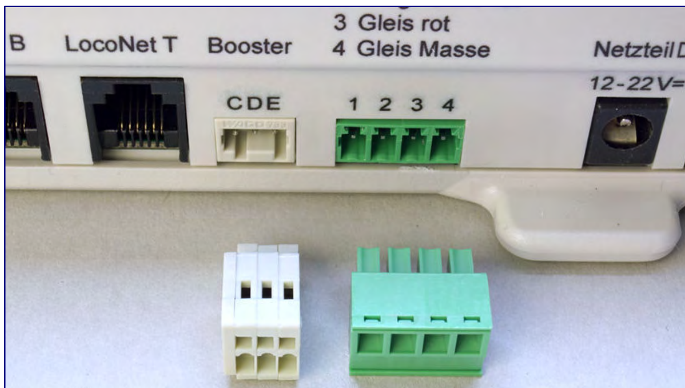
The necessary plugs for connecting DC boosters and tracks for operating and programming are included with the Intellibox 2neo.
